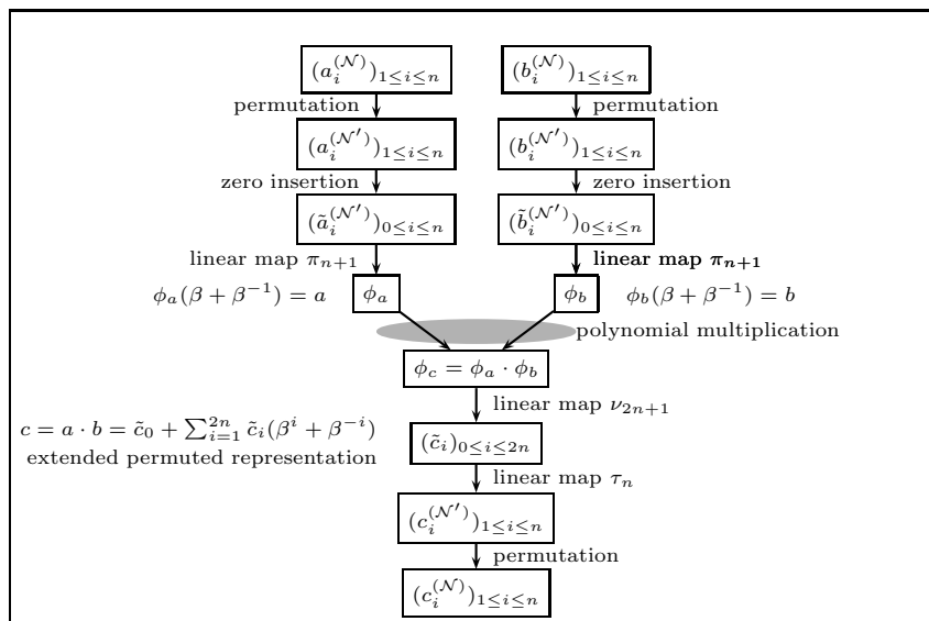
Fig. 1. Overview of our multiplier structure to multiply two elements a, b \in \mathbb{F}_q^n in the representation (*_i^{(\mathcal{N})})_{1 \leq i \leq n} with respect to the normal basis \mathcal{N}
