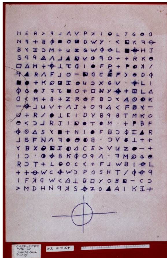
Figure 1: Zodiac-340 ciphertext. 1
